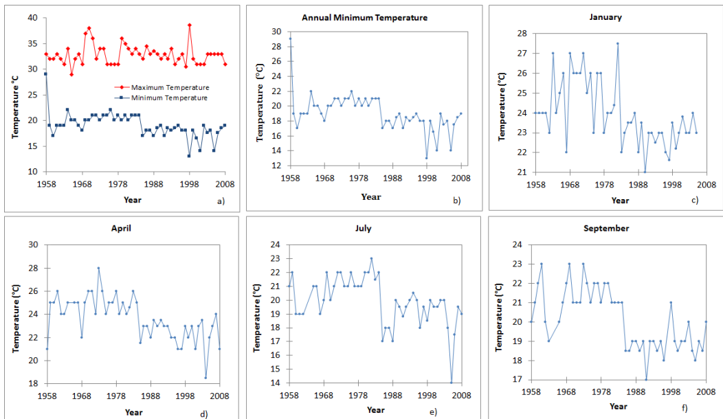
Figure 5. Behavior of the annual maximum and minimum temperature (a); minimal annual (b); and minimum for the central months of the seasons of the year (c, d, e, f).
