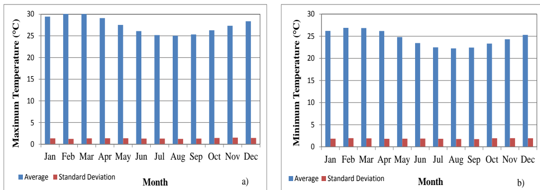
Figure 3. Basic descriptive statistics regarding the average and dispersion of maximum (a) and minimum (b) temperatures in the Trindade Island, South Atlantic.
