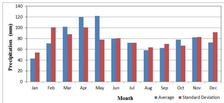
Figure 2. Mean and standard deviation of monthly rainfall for the historical time series from 1984 to 2008.
