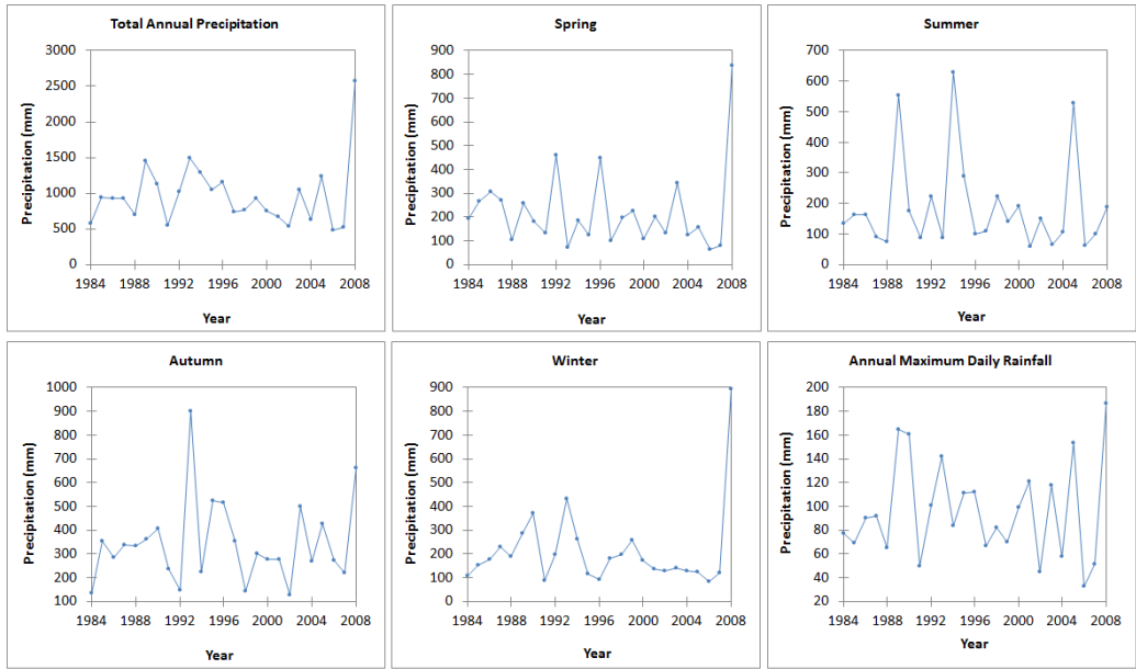
Figure 4. Temporal distribution of rainfall on Trindade Island, tropical South Atlantic Ocean.
