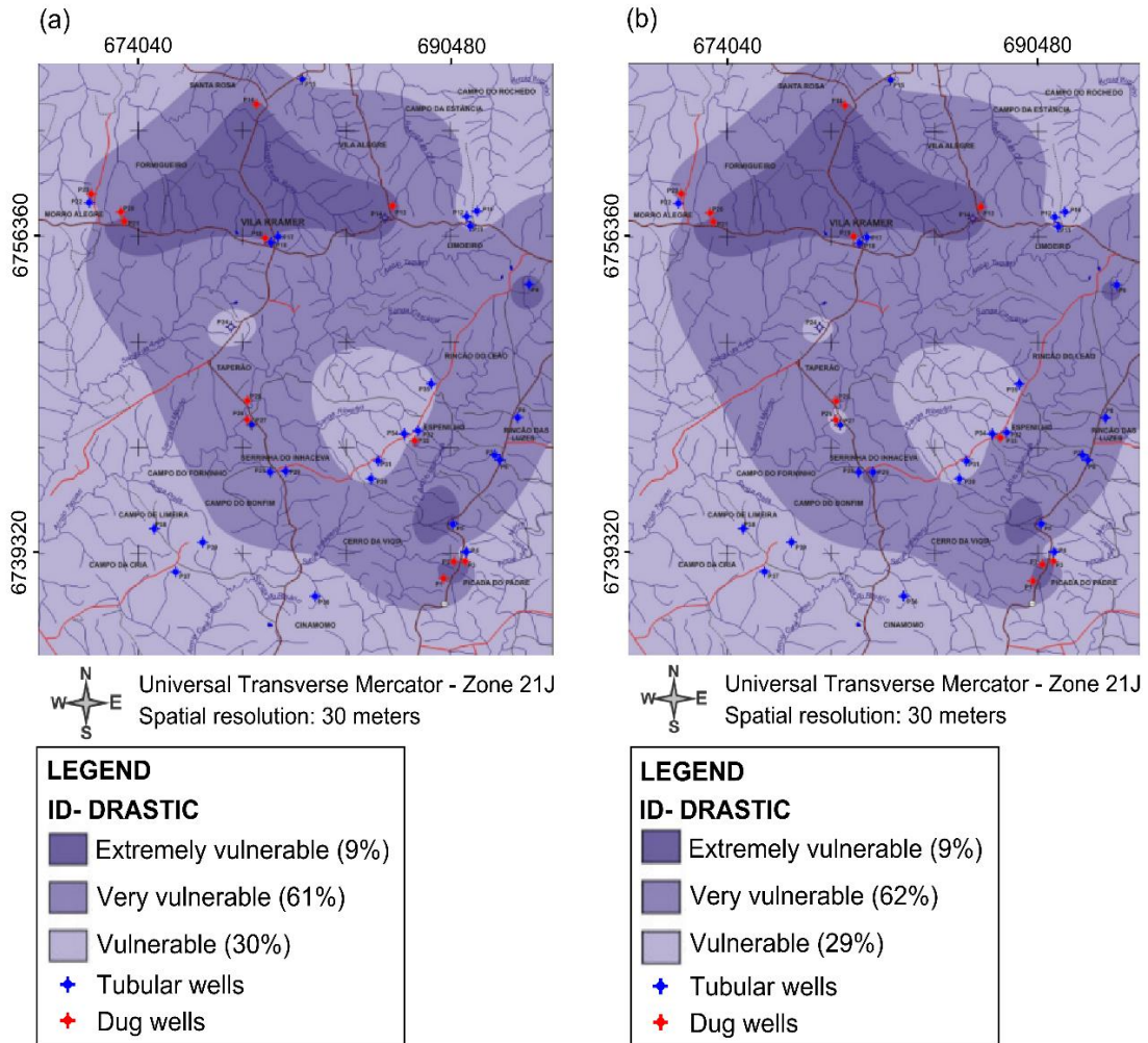
Figure 3 - Groundwater contamination vulnerability maps obtained by the DRASTIC model with S parameter on the 1:50.000 (a) and 1:1.100.000 (b) scales.
